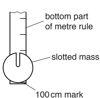
Fig. 2.2 (front view)
