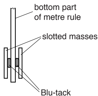
Fig. 2.3 (side view)
